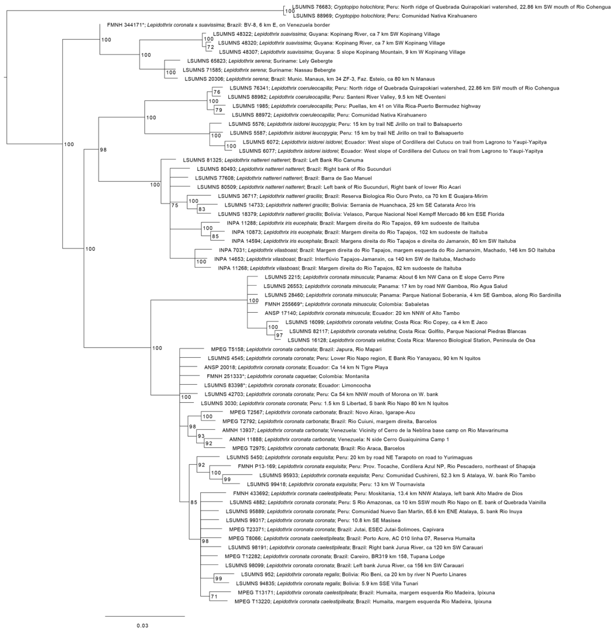
Figure S1. Phylogenetic estimate of the genus Lepidothrix in IQ-TREE using the “linked”, 75% complete SNP dataset (5025 parsimony-informative SNPs). This is the same tree as that in Figure 1 but with further sample information and with outgroups displayed. The four toepad samples are denoted with an asterisk. Branch support given by bootstrap values, and all branches with a value <70 are collapsed to a polytomy.
