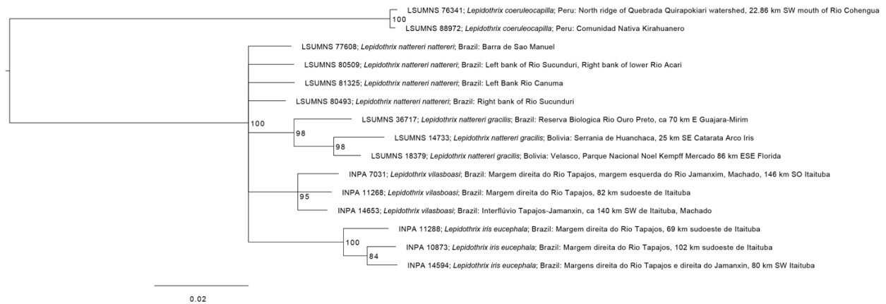
Figure S10. Phylogenetic estimate of the Lepidothrix nattereri + L. vilasboasi + L. iris clade in IQ-TREE using the “unlinked”, 95% complete SNP dataset (622 parsimony-informative SNPs). Branch support given by bootstrap values, and all branches with a value <70 are collapsed to a polytomy.
