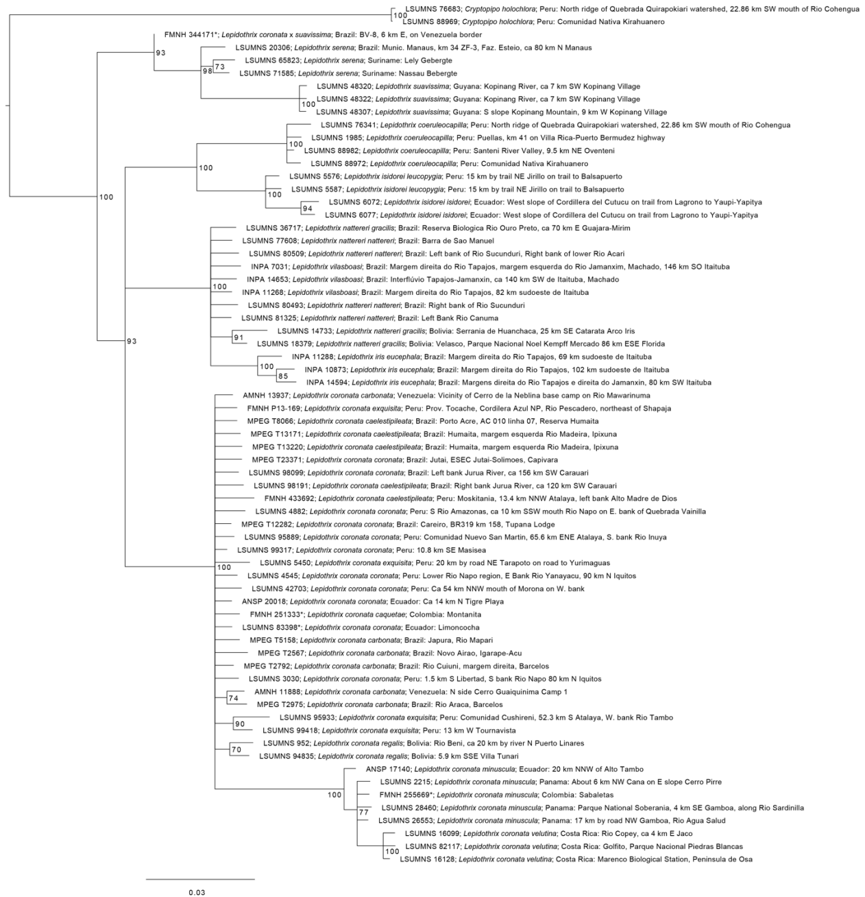
Figure S4. Phylogenetic estimate of the genus Lepidothrix in IQ-TREE using the “unlinked”, 95% complete SNP dataset (1120 parsimony-informative SNPs). The four toepad samples are denoted with an asterisk. Branch support given by bootstrap values, and all branches with a value <70 are collapsed to a polytomy.
