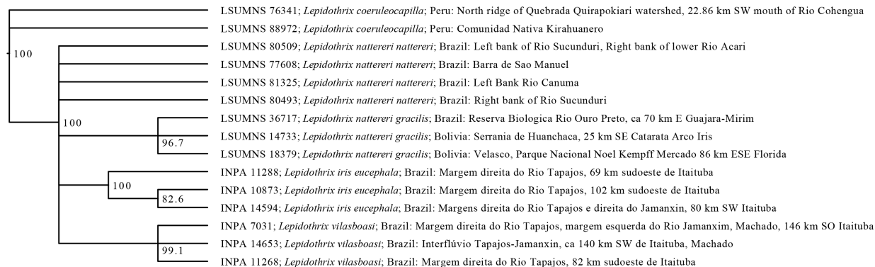
Figure S11. Phylogenetic estimate of the Lepidothrix nattereri + L. vilasboasi + L. iris clade in SVDquartets using the “unlinked”, 75% complete SNP dataset (1363 SNPs). Branch support given by bootstrap values, and all branches with a value <70 are collapsed to a polytomy.
