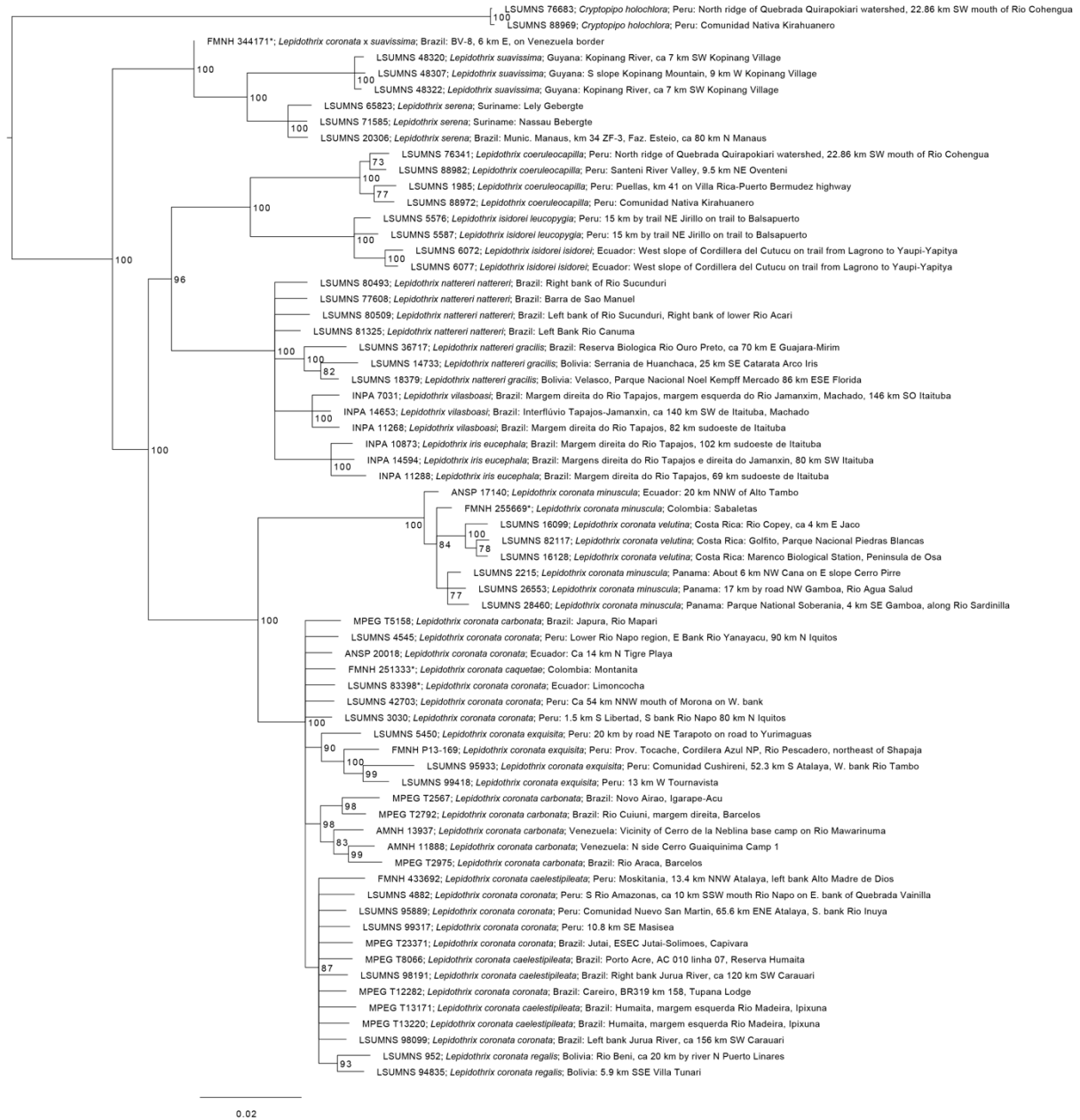
Figure S2. Phylogenetic estimate of the genus Lepidothrix in IQ-TREE using the “linked”, 95% complete SNP dataset (4041 parsimony-informative SNPs). The four toepad samples are denoted with an asterisk. Branch support given by bootstrap values, and all branches with a value <70 are collapsed to a polytomy.
